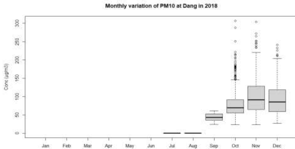
Figure 12: Monthly Variation of PM 10
