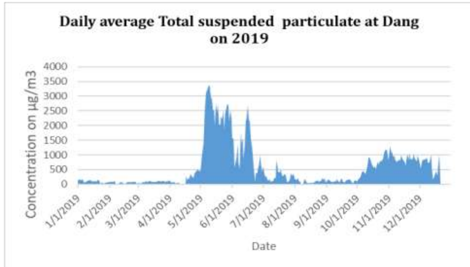
Figure 42: Daily Average of TSP
