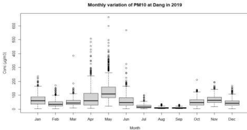
Figure 37: Monthly Variation of PM 10
