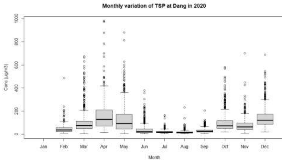
Figure 72: Monthly Variation of TSP
