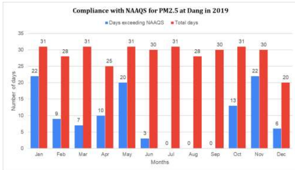
Figure 33: Compliance Status of PM 2.5
