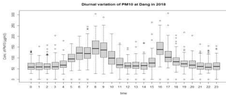
Figure 13: Diurnal Variation PM 10
