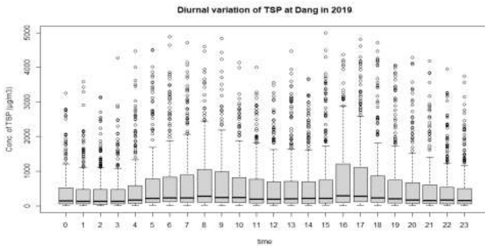
Figure 46: Diurnal Variation of TSP
