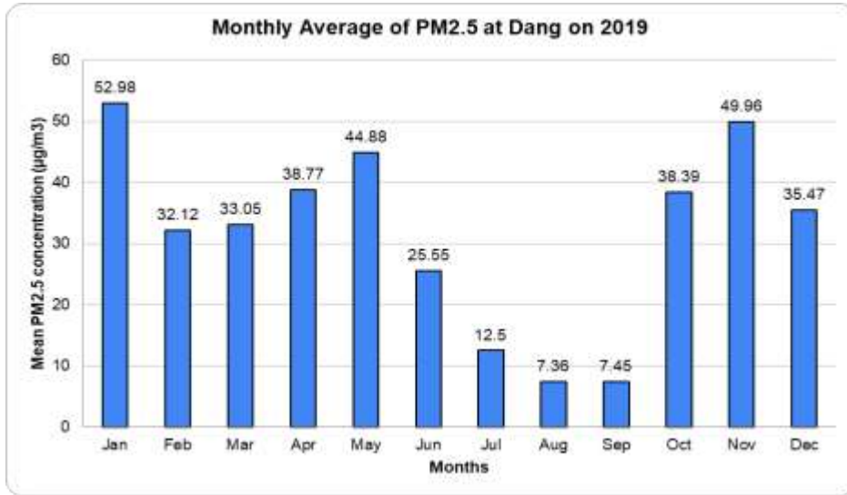
Figure 29: Monthly Average of PM 2.5
