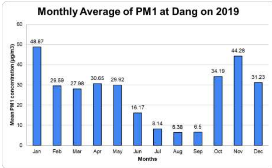
Figure 23: Monthly Average of PM 1
