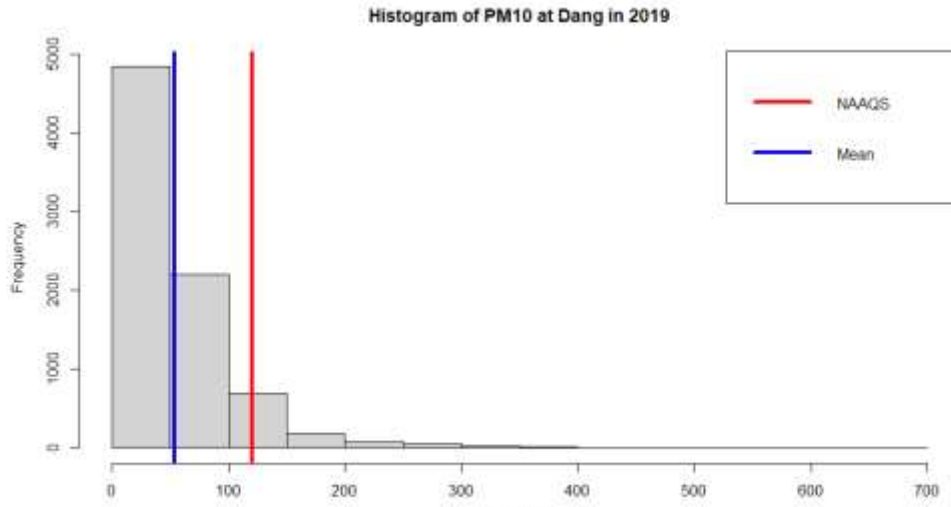
Figure 34: Histogram of PM 10
