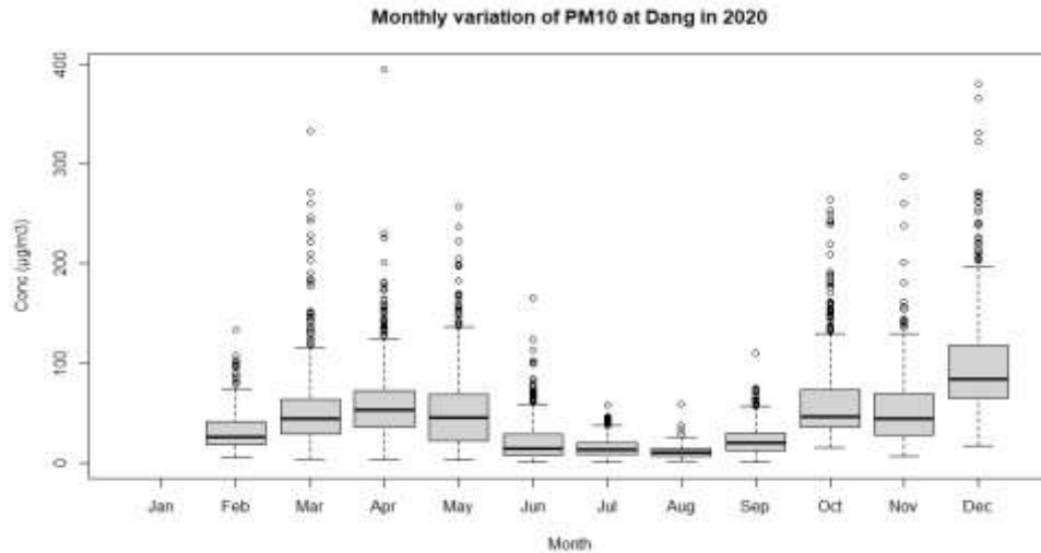
Figure 65: Monthly Variation of PM 10
